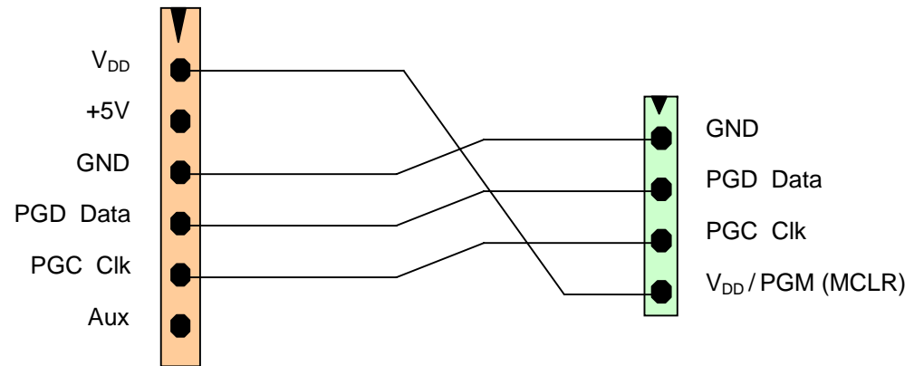
PICKIT to G4JNT In-Circuit Programming Interface
