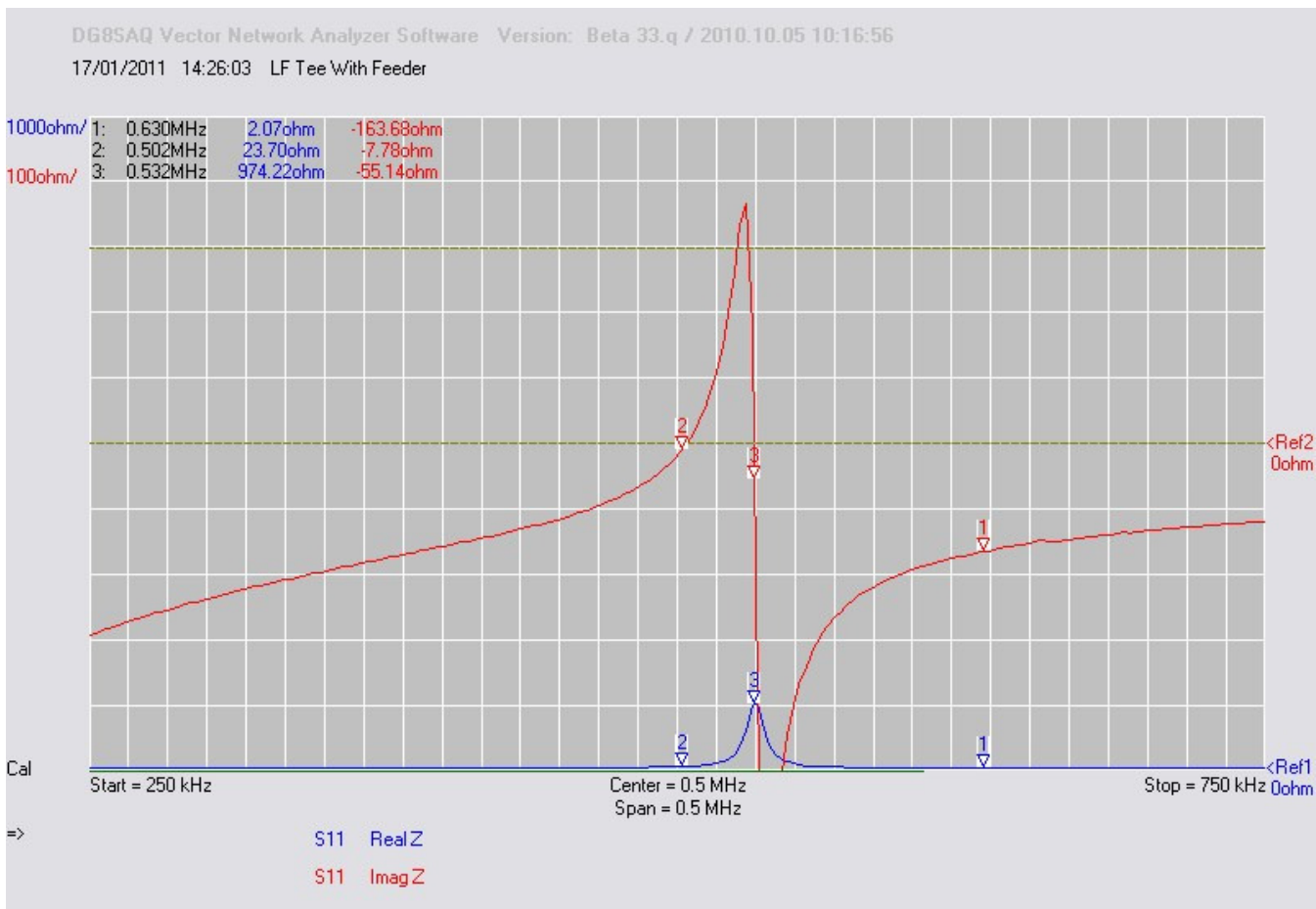
500kHz Tee antenna + loading coil measured at base (upper plot) and through 12m of UR43 (lower )
